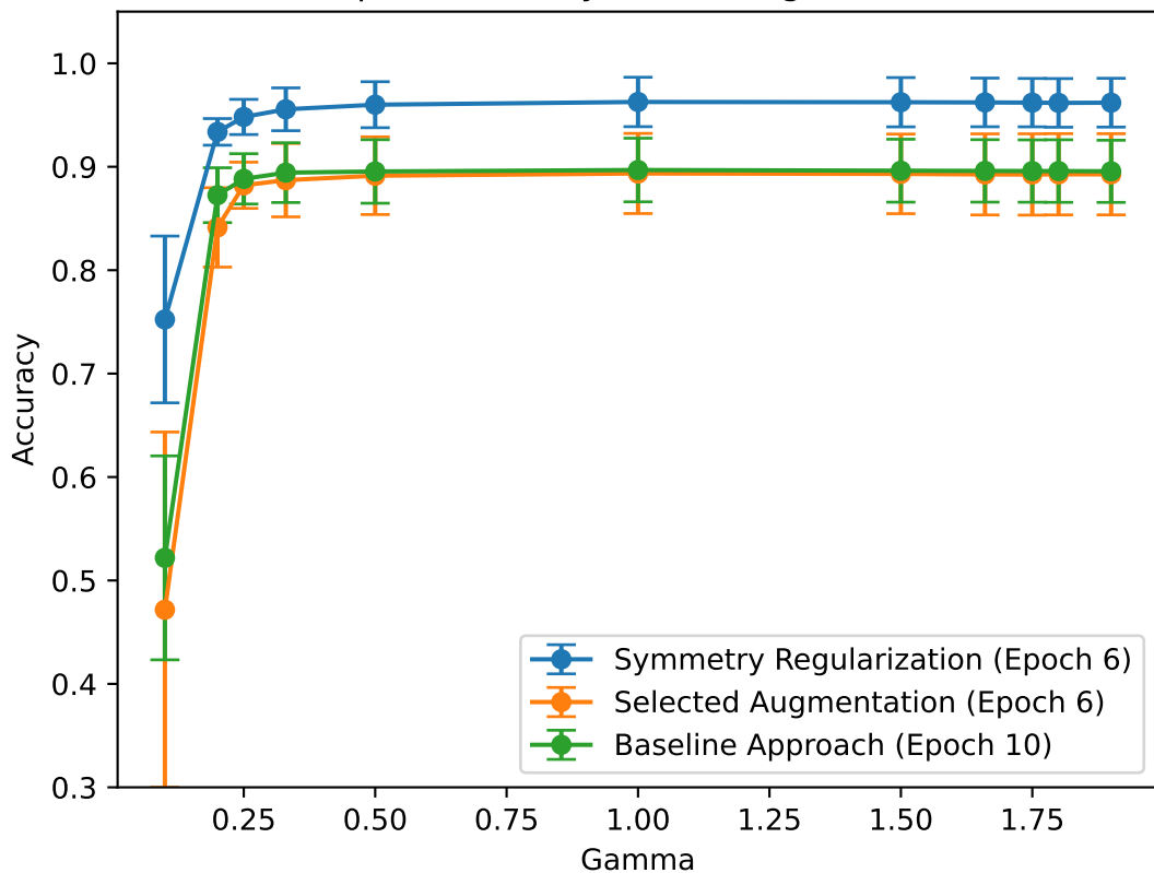
Accuracies at Epochs directly before Regularization is Matched
